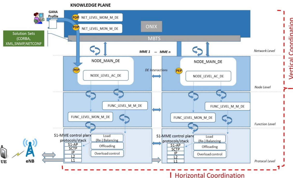
Figure 11: Instantiation of DEs and indicative parameters in the MME pooling management example
