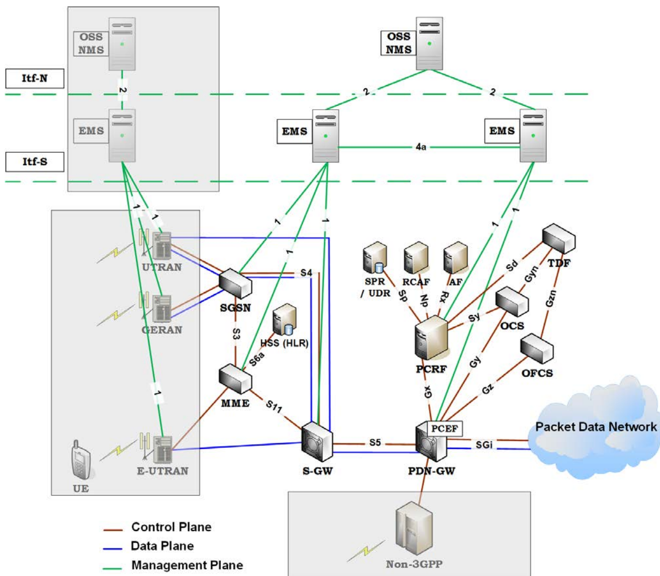
Figure 3: Management plane for the non-aggregated scenario
