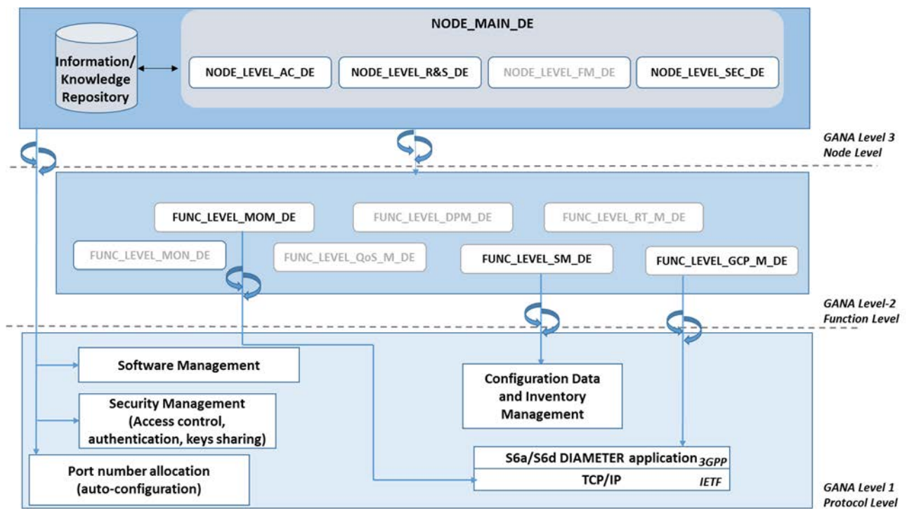
Figure 7: Node level view of Self-configuration case for the HSS
