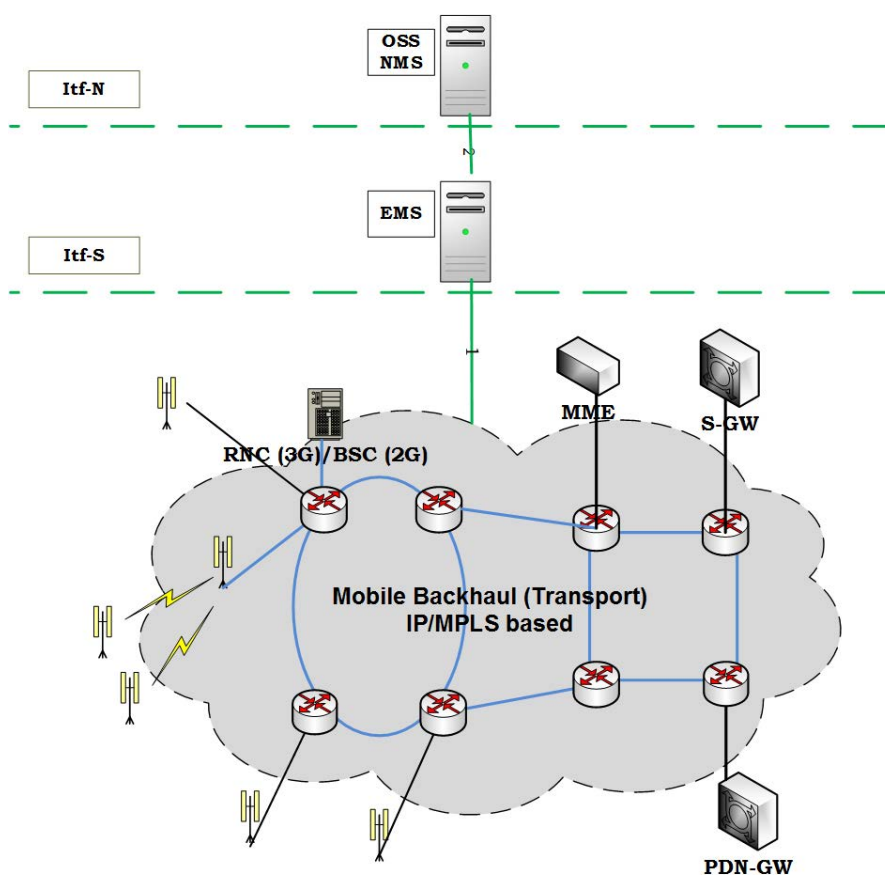
Figure 4: Reference architecture for the backhaul
