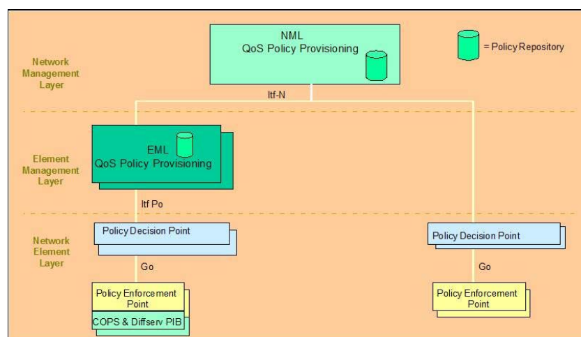
Figure 5: Conceptual architecture for a policy-based QoS Management System (reproduced from ETSI TS 132 101 [i.30])
