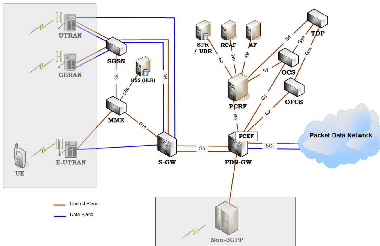
Figure 2: Reference 3GPP architecture
