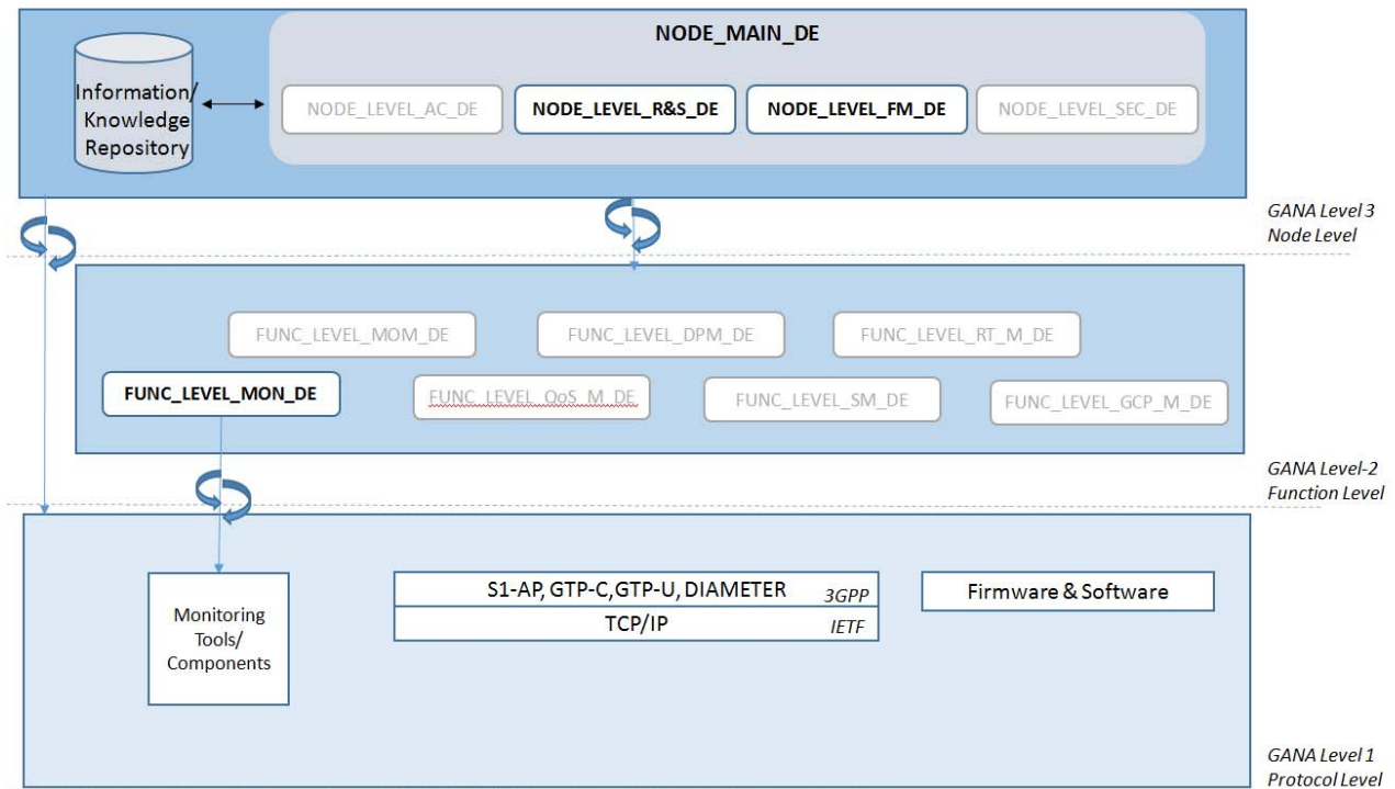
Figure 13: Node level view of self-healing case for the P-GW
