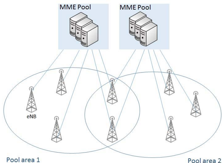
Figure 9: MME pooling concept
