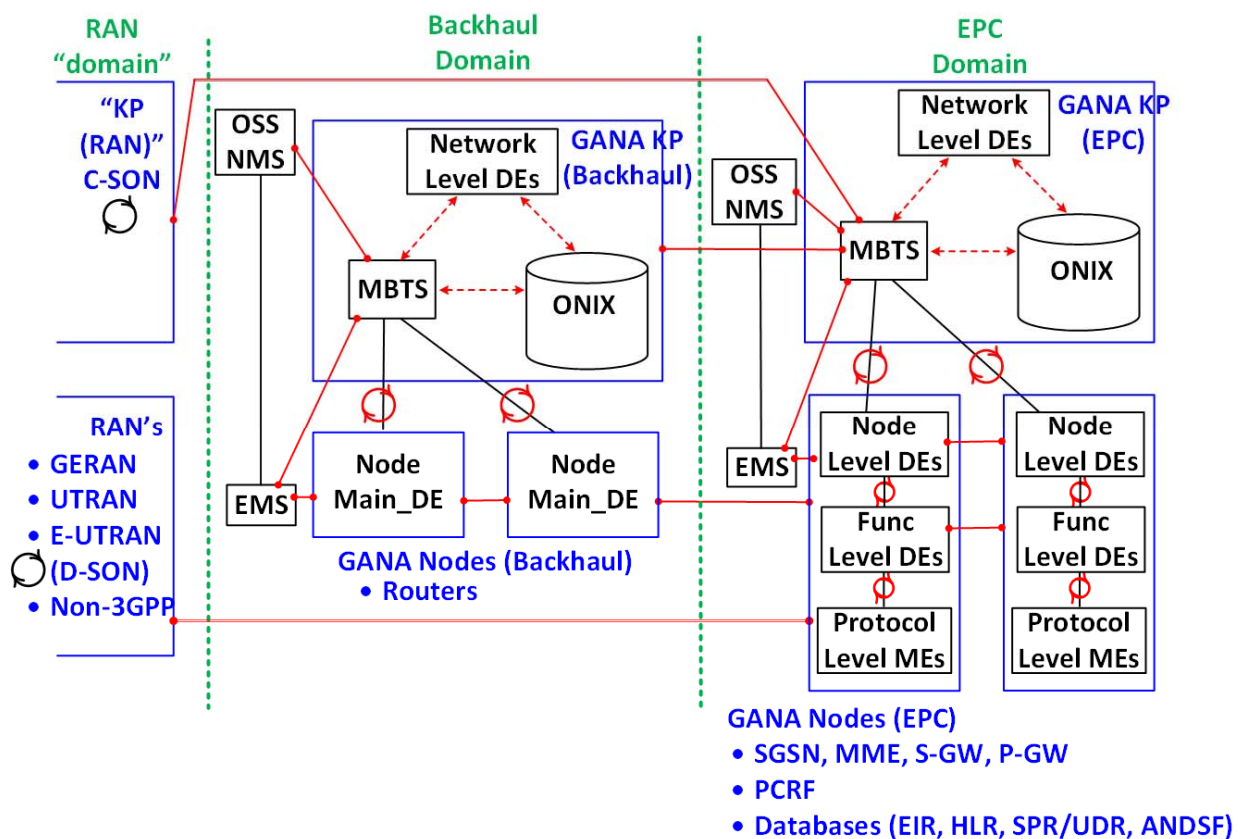
Figure 18: Interactions involving GANA entities for 3GPP Core Network and backhaul mapping
