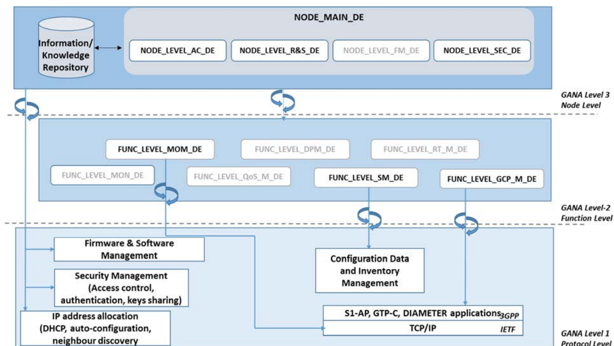
Figure 6: Node level view of Self-configuration case for the MME
