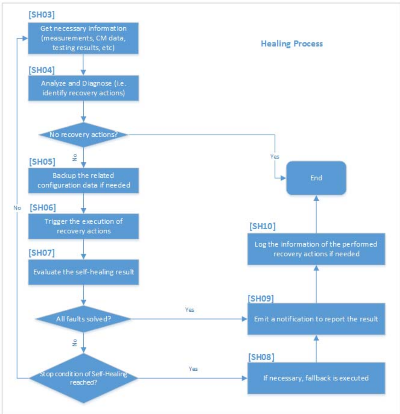
Figure 15: Self-healing processing part
