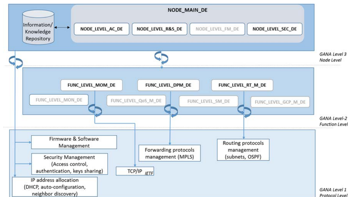
Figure 8: Node level view of Self-configuration case for a router of the backhaul network
