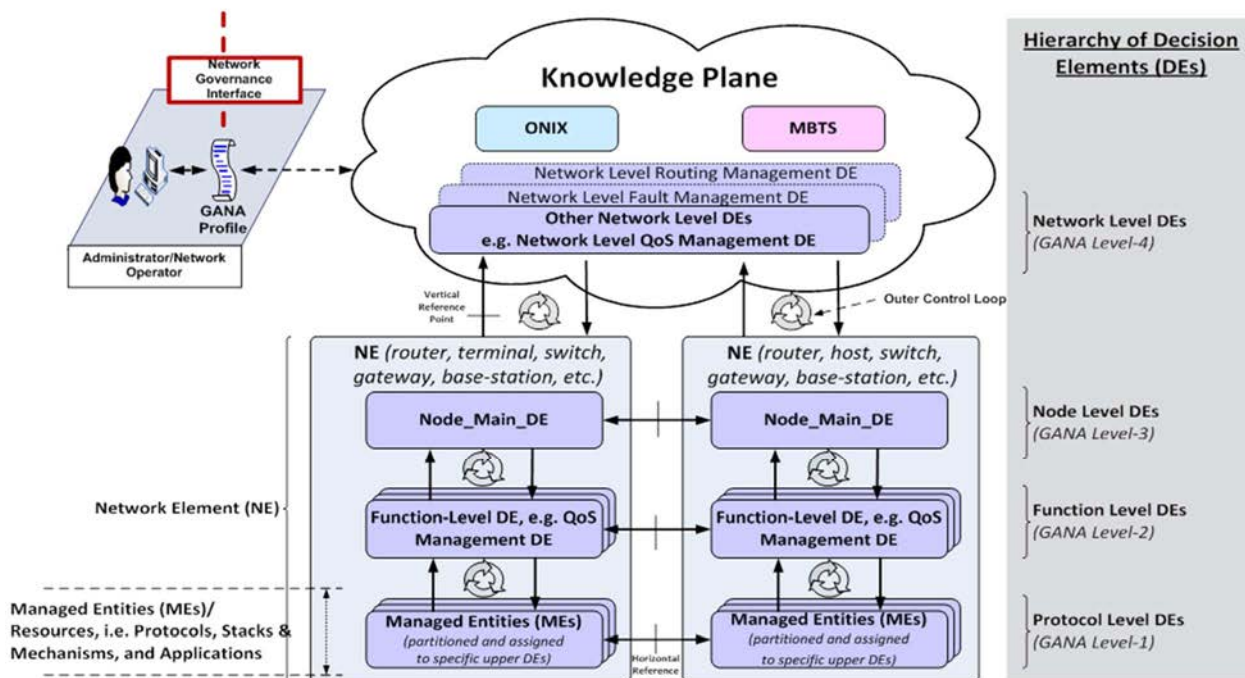
Figure 1: Snapshot of the AFI GANA Reference Model
