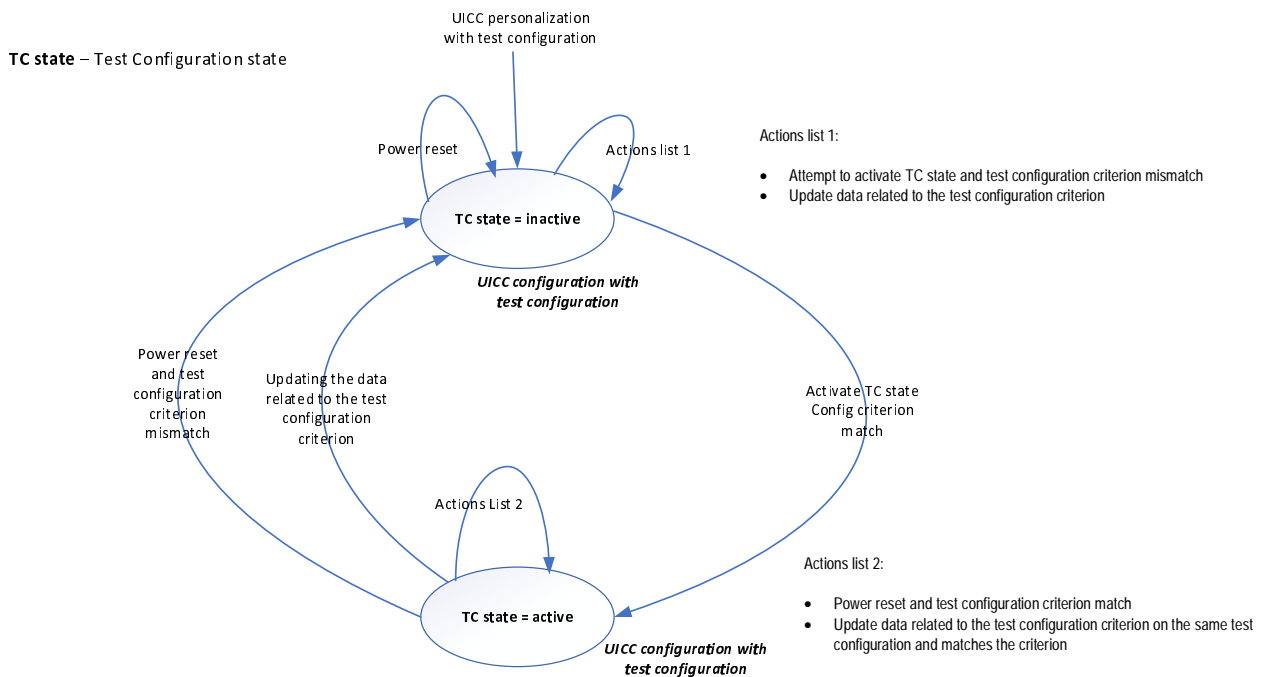
Figure N.1: State transitions of test configuration state on a UICC with a test configuration
